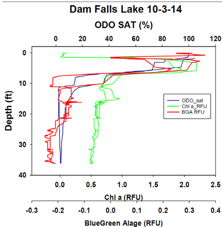
Figure 8. Depth profile of Falls Lake October 2014 that shows the subsurface algae maximum around 10-15 feet and the ammonium nutrient flux from the anoxic bottom sediments.
