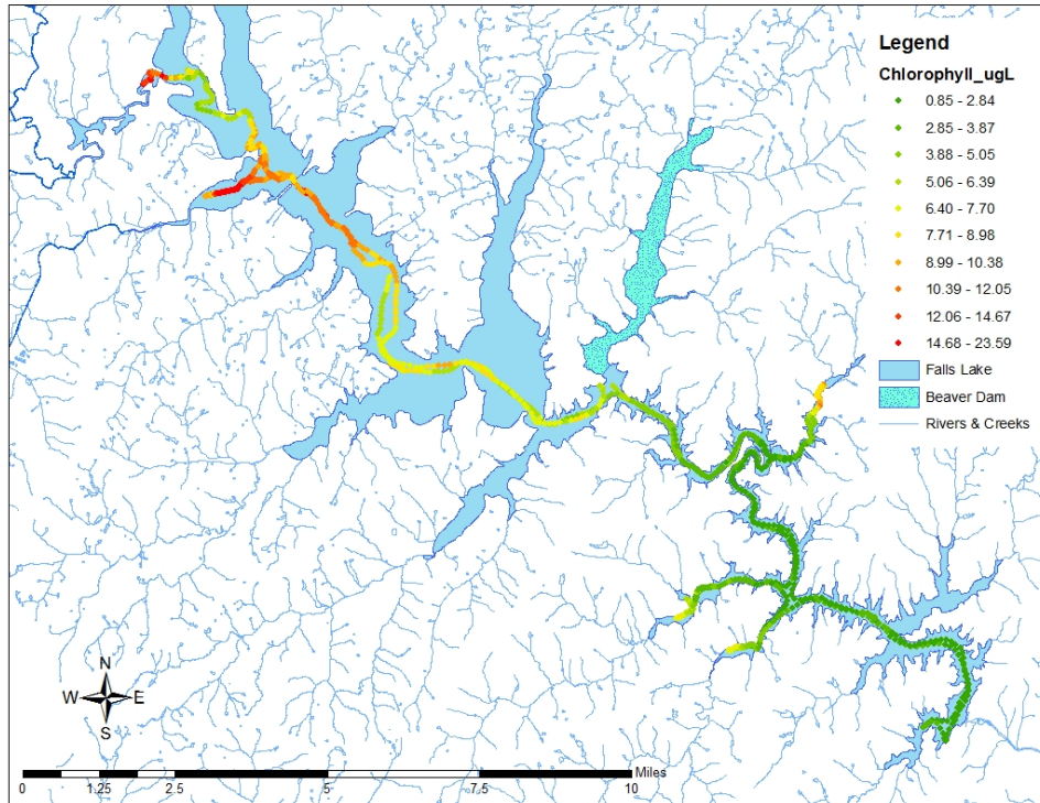
Figure 7. Chl a map of Falls Lake August 2014. Chl a concentrations are elevated in the shallow northern portions of the lake. Water is withdrawn for Raleigh Drinking water in the lower portion of the lake where surface Chl a concentrations are low.
